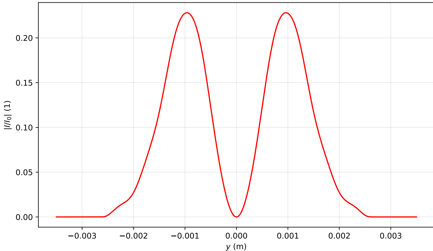
Intensity profile I(x=0, y, z=3.503)/I_0 , P_{in}=1.0P_{cr} , artificial time
